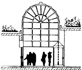
9 Plan, elevation and detail of barrel roof → 12
